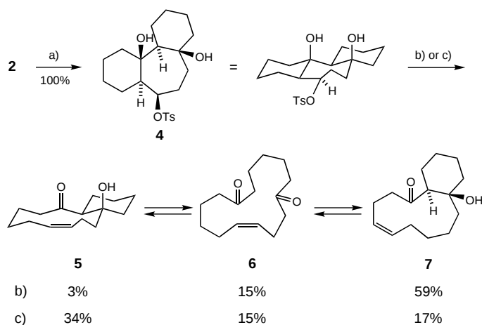
Scheme 4. Grob fragmentation of tosylate 4 : a) n\text{BuLi} (1.5 equiv), \text{TsCl} (1.15 equiv), THF, -15^\circ\text{C} , 20 min; b) \text{KOtBu} (3 equiv), t\text{BuOH} , THF, -6 to 0^\circ\text{C} , 25 min; c) \text{KOtBu} (3 equiv), DMF/THF (3:2), 0 to 15^\circ\text{C} , 15 min.
