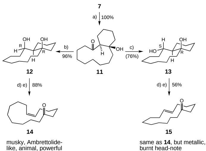
Scheme 6. Syntheses of ( Z )-6- and ( E )-6-cyclopentadecenones 14 and 15 : a) \text{H}_2 , Pd (10%)/C, cyclohexane; b) \text{LiAlH}_4 (1.2 equiv), \text{Et}_2\text{O} , RT; c) Red-Al® (4.0 equiv), THF, -78^\circ\text{C} to room temperature; d) n\text{BuLi} (1.5 equiv), \text{TsCl} (1.15 equiv), THF, -15^\circ\text{C} , 20 min; e) \text{KOtBu} (3 equiv), t\text{BuOH} , 25\text{--}31^\circ\text{C} , 10 min.
