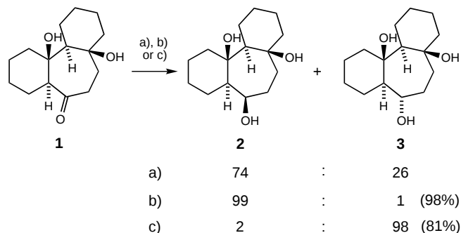
Scheme 3. Diastereoselective reductions of ketone 1 . a) LiAlH 4 (1.15 equiv), THF, -70 °C to -50 °C; b) Red-Al® (3.0 equiv), THF, -70 °C to room temperature; c) BH 3 ·SMe 2 (0.71 equiv), THF, room temperature.
